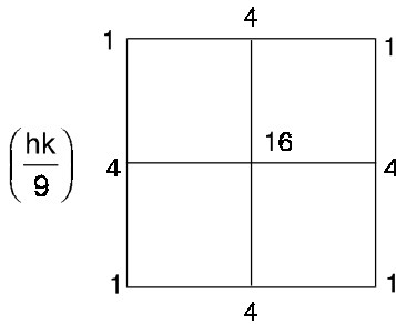
Simpson's rule
