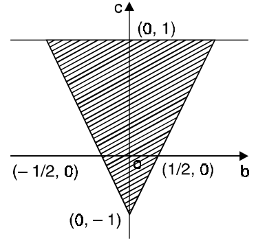
Fig. 5.2. Stability region
